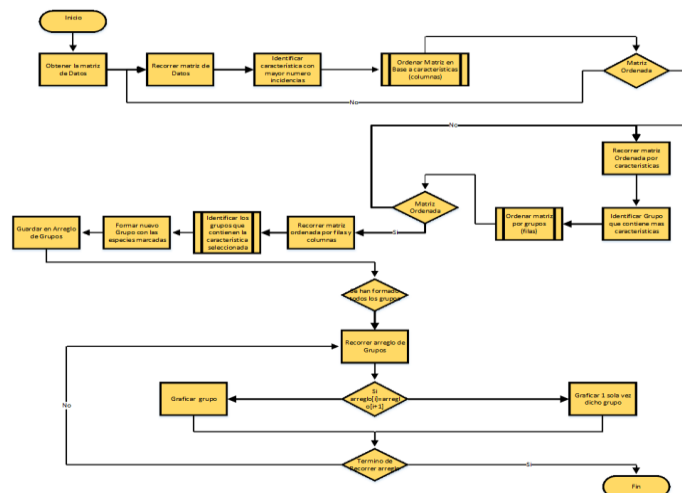
Figure 8 Hennig Flowchart
